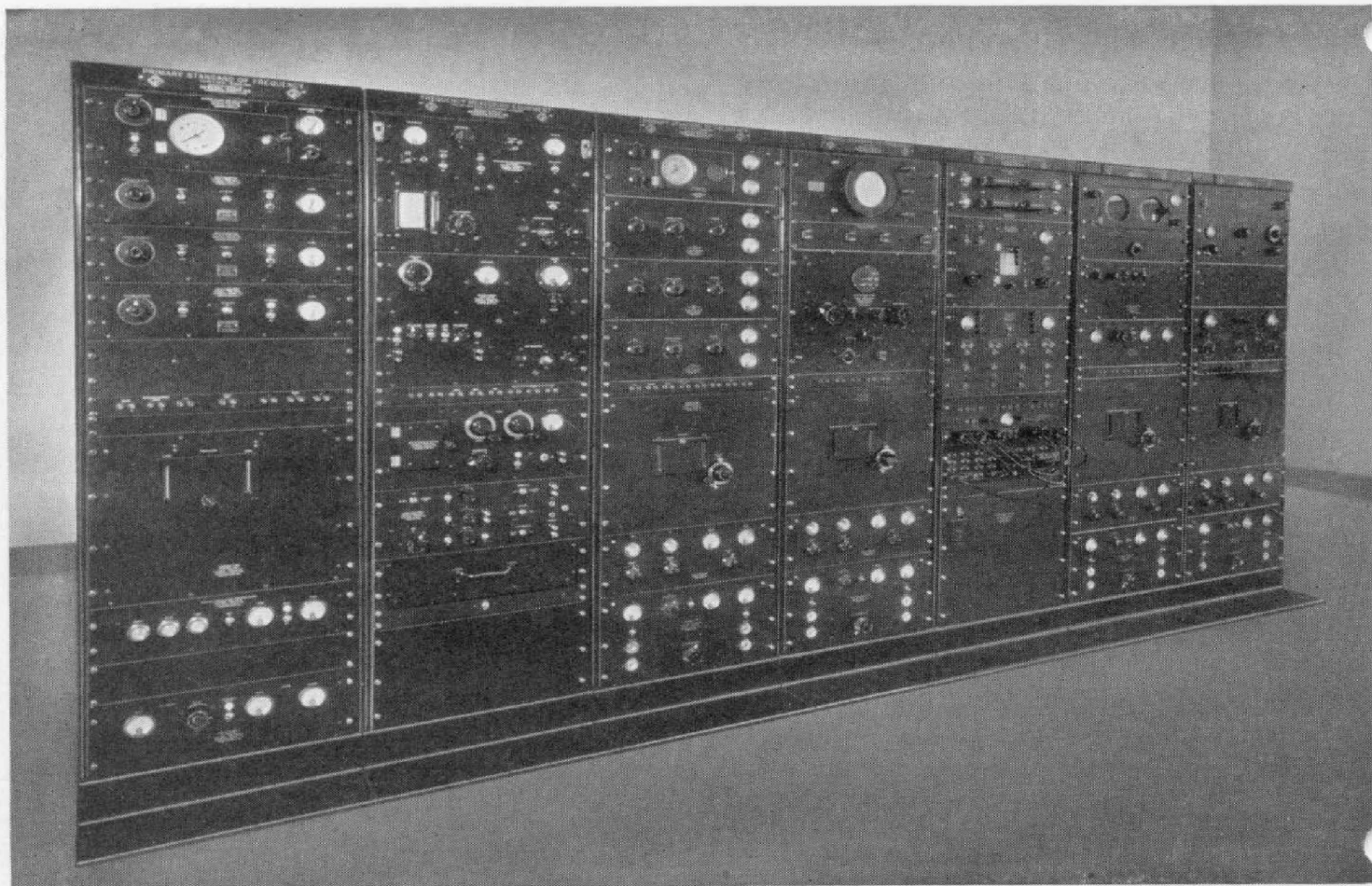
FIGURE 1. The primary frequency standard at General Radio Company
