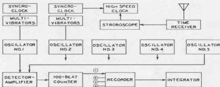
FIGURE 3. Block diagram of the primary standard. For convenience, only one beat recording channel is shown in detail. Beats between Oscillator No. 5 and each of Nos. 2, 3, and 4 are counted and recorded in the same way
